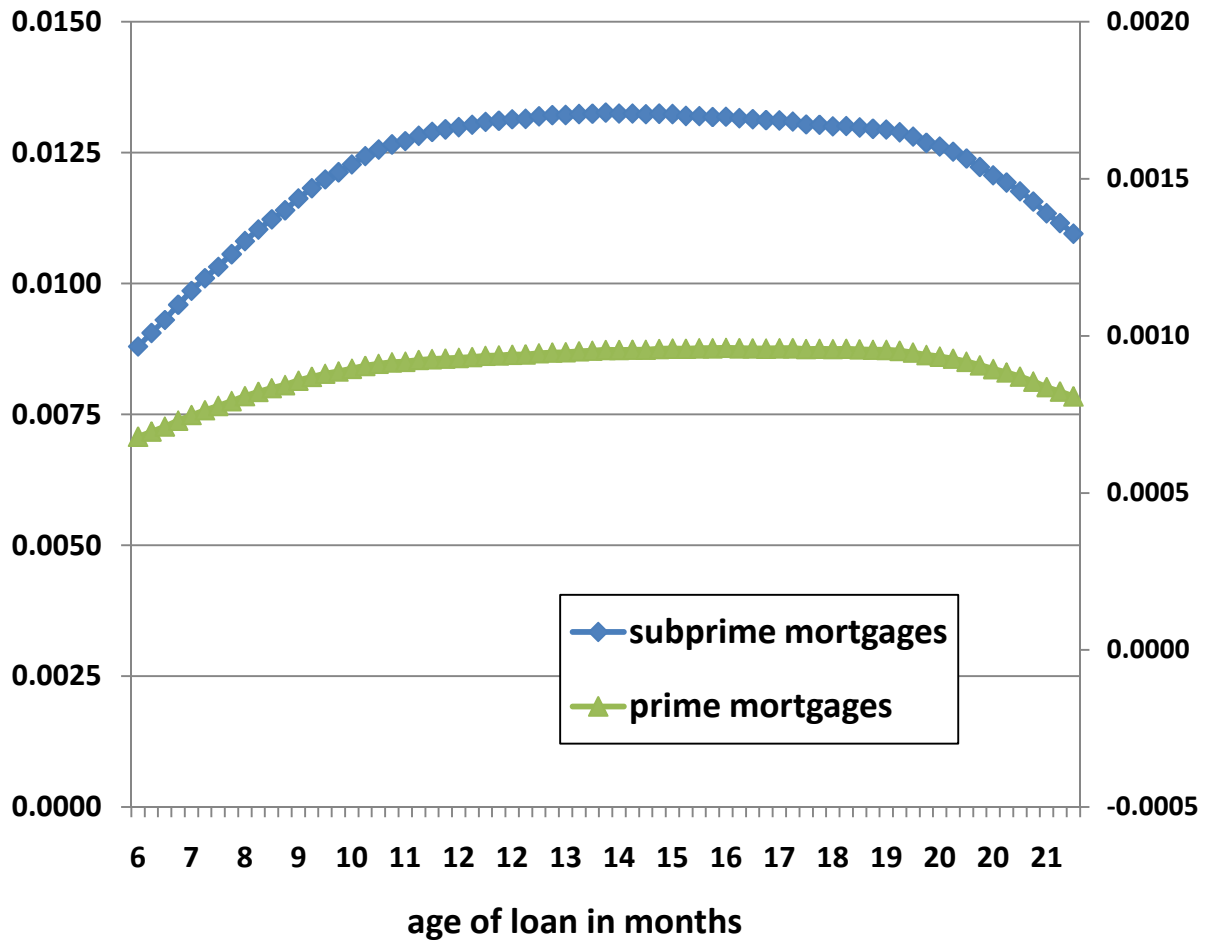
Baseline Default Hazard As a Function of Mortgage Age
